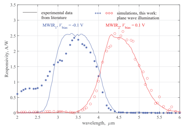
Fig. 2. 3D MWIR 1 -MWIR 2 simulated spectral responsivity for plane wave illumination (symbols) compared with the experimental values from [4, Fig. 2].
