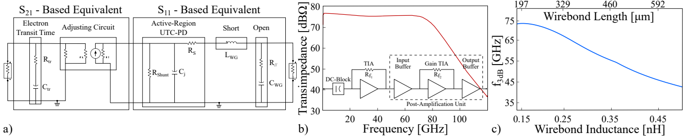
Fig. 2. a) Full equivalent circuit of a UTC-PD; b) block diagram and transimpedance of the TIA; c) 3dB-Bandwidth of the mm-wave device.
