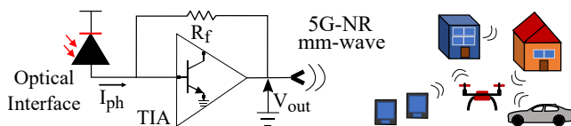
Fig. 1. A mm-wave transmission component combining a UTC-PD, a TIA and an antenna element transmitting 5G-NR based signals to various end-users.
