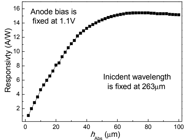
Fig. 4. Responsivity as a function of h_{Abs} with the anode bias fixed at 1.1\text{V} and the incident wavelength fixed at 263\mu\text{m} .
