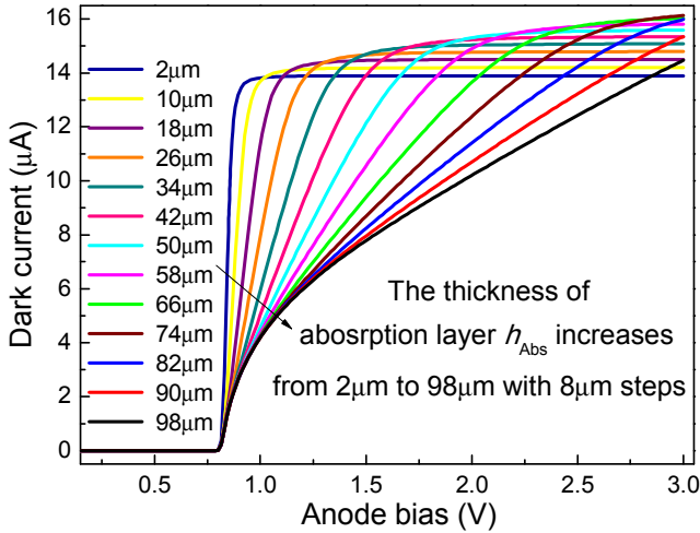
Fig. 2. Dark current versus anode bias with the thickness of the absorbing layer ( h_{Abs} ) increasing from 2\mu\text{m} to 98\mu\text{m} in 8\mu\text{m} steps.
