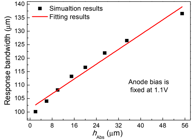
Fig. 5. Fitting result of response bandwidth ( BW_R ) versus h_{Abs} with the anode bias fixed at 1.1V.
