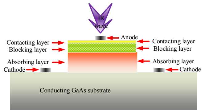
Fig. 1. Schematic of structural model for GaAs-based BIB detector.
