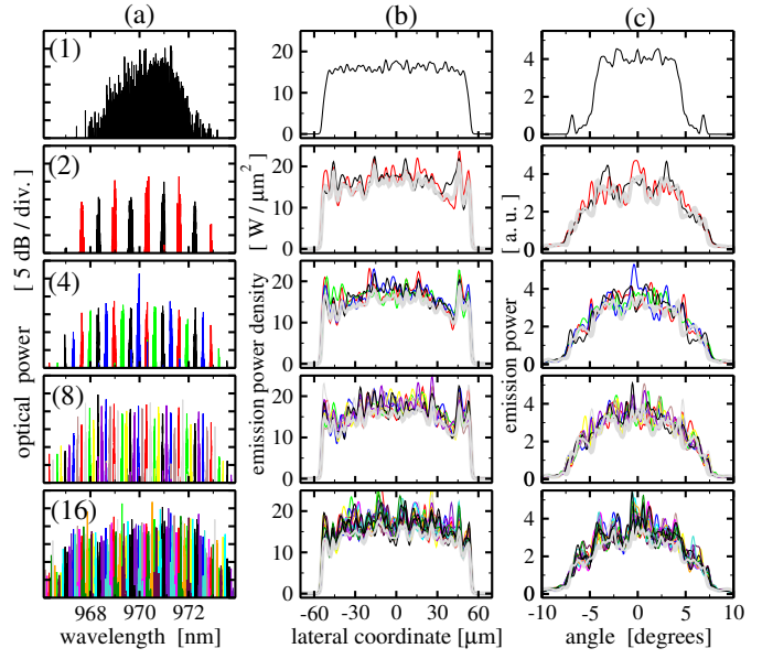
Fig. 3. Simulations of the single diode without feedback (1) and 2/4/8/16 coupled BALs (corresponding lower rows). Thin lines: optical spectra (a) and field intensities (b) of the individual diode emission at the front facet, as well as corresponding far fields (c). Thick grey in (b) and (c): representations of the combined beam (divided by the number of emitters) at the F_{out} plane.
