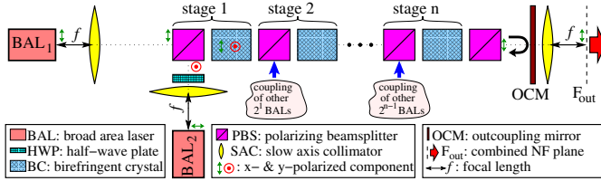
Fig. 1. Schematics of 2^n BALs coupled by the cascaded external cavity with n stages. Coupling of the first two diodes within Stage 1 is shown explicitly.
