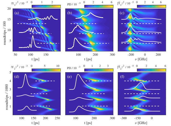
Figure 2. (a,d) Space-time diagrams for the intensity of a passively mode-locked VECSEL. (b,e) Low pass filtered time trace @10 GHz in order to emulate finite Photodetector bandwidth. (c,f) Single shot optical spectrum. (a,b,c) and (d,e,f) correspond to two different parameters set, and the satellites pulsating on the front of the pulse can take different shapes as a function of the effective amount of TOD
