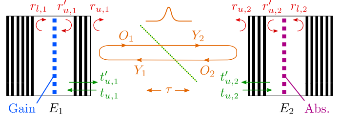
Figure 1. A schematic of the coupled cavities configuration. E_j denote the intra-cavity fields, j = 1, 2 . The output and input fields in the external cavity are represented by O_j and Y_j , respectively. The time of flight in the cavity is \tau .
