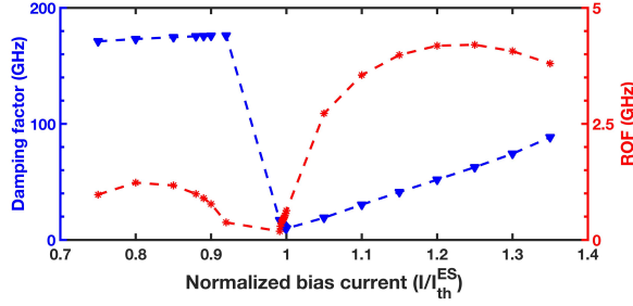
Fig. 2. Current dependence of damping factor (blue) and relaxation oscillation frequency (red).
