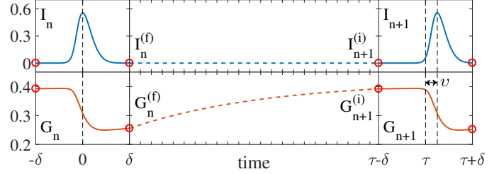
Figure 1. Temporal profile of the intensity I_n = |A_n|^2 and of the gain G_n at the n -th and n+1 -th round-trips. After the emission of the pulse I_n and the ensuing gain depletion, the so-called fast stage (solid lines), the gain recovers until the next round-trip while the field is vanishing (dashed lines). Knowing the final value of G_n^{(f)} in the interval z \in [-\delta, \delta] , one can deduce the initial gain value at the next round-trip G_{n+1}^{(i)} . The central panel is not up to scale and can be several orders of magnitude larger than the outer panels.
