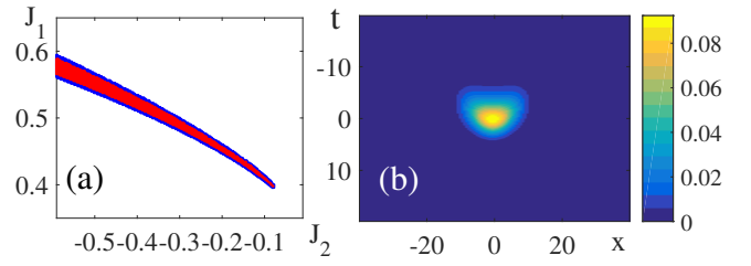
Figure 2. (a) Two-dimensional bifurcation diagram showing the region of stable existence of the LBs of the DAE model (5-7) as a function of the reverse bias in the gain and absorber sections J_1 and J_2 . (b) Spatio-temporal profile of the field found with the FM with (J_1, J_2) = (0.498, -0.336) . Other parameters are (\alpha_1, \alpha_2, h, \gamma_1, \gamma_2, s, \eta) = (0, 0, 2, 0.003, 0.1, 30, 0.5) .
