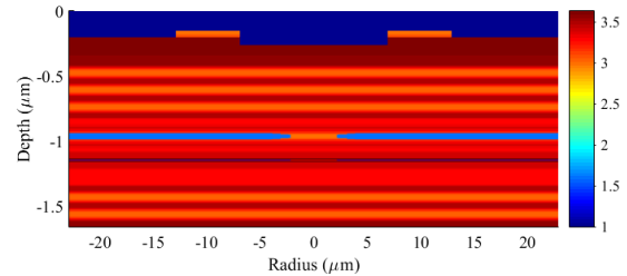
Fig. 1: Refractive index transverse section of the optical structure in a compact form (DBR multiplicity skipped) of investigated VCSEL [7]. Blue region ( n = 1 ) indicates air; the two relieves at the top are the metal contact placed above the a p^{++} -doped GaAs layer; the region between two light blue stripes is the oxide aperture. Below the QW region. The 110nm thick substrate is not shown.
