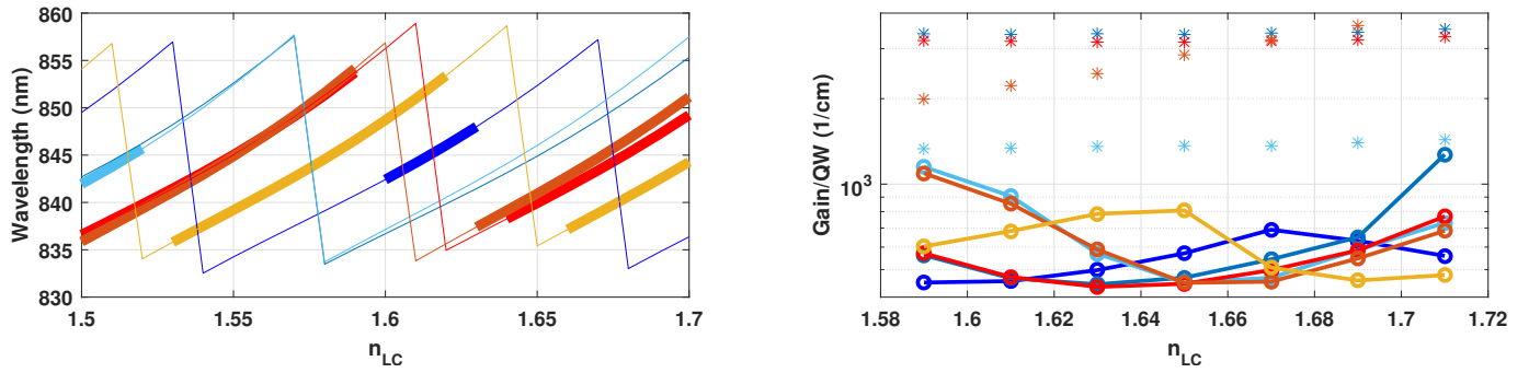
Fig. 2: Output results of the LC-VCSEL VELM simulation varying the SU-8 alignment layer thickness (warm [500 nm] to cold [700 nm] colours) and the LC reservoir (from darker [2800 nm] to lighter [3200 nm] colours). On the left: 1D tuning curves. Thick lines represent the range for which extraordinary emission prevails on the ordinary. On the right: 3D gain thresholds comparison between ordinary (asterisks) and extraordinary modes (line with circle). The y axis has been clamped to put in evidence the details of the extraordinary threshold gain.
