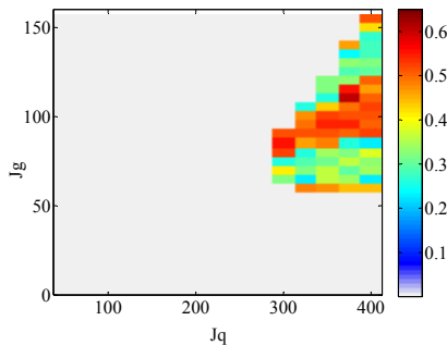
Fig. 5. The rms-timing jitter of intra-cavity long ring laser that is normalized to the rms-timing jitter of the fundamental(20GHz) ring laser.
