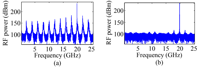
Fig. 3. Electrical spectrum (RBW=1 MHz) of tenth harmonic of without-intracavity (a) and with-intracavity long ring laser (b).
