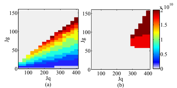
Fig. 2. Dynamic of repetition frequency for without-intracavity (a) and with-intracavity long ring laser (b).
