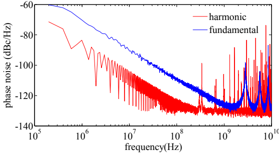
Fig. 4. The single side-band phase noise of the fundamental(20GHz) ring laser and the tenth harmonic of intracavity long ring laser .
