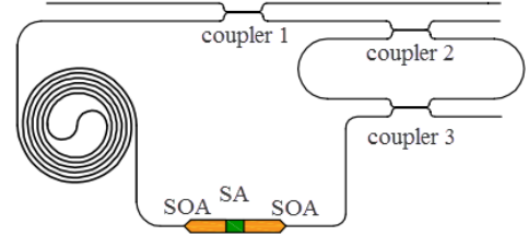
Fig. 1. Schematic of Mode-Locked hybrid silicon laser with intracavity Filter. Black lines indicate passive Si waveguides [1,5]. SOA—Semiconductor optical amplifier, SA—saturable absorber
