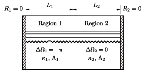
Fig. 1 Schematic structure of a coupled cavity DFB-LD with phase-shifted/uniform gratings.
