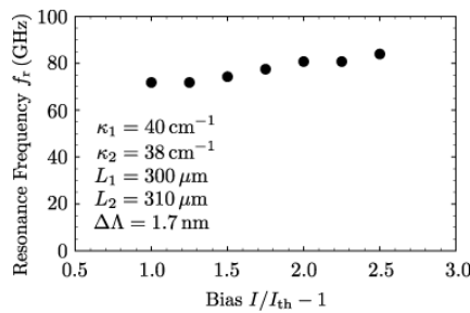
Fig.3 Resonance frequency f_r as a function of I/I_{th}-1 .
