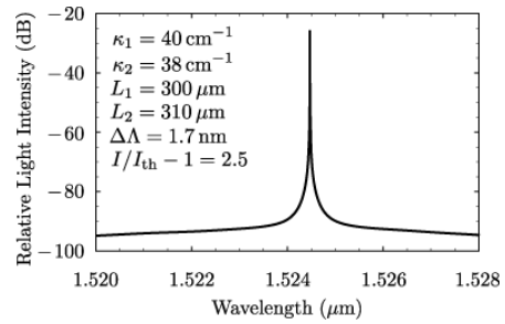
Fig.5 Oscillation spectrum.
