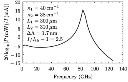
Fig.4 Frequency response.
