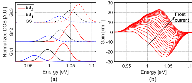
Fig.2. Simulations. (a) Normalized DOS in the three chirped QD layer for GS, ES 1 and ES 2 . (b) Gain at the front facet for a 120 mA rear electrode current and a front electrode current uniformly varied from 160 mA to 5 A.
