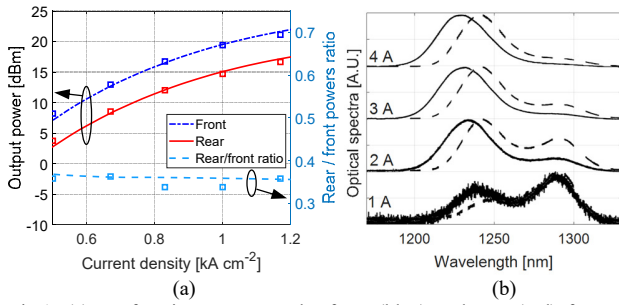
Fig.1. (a) Left axis: powers at the front (blue) and rear (red) facets; simulations (continuous line) and experiments (markers). Right axis: ratio of the rear and front facet powers; simulations (dashed line) and experiments (markers). (b) Experimental optical spectra at the front (continuous) and rear (dashed) facets for front facet currents from 1 A to 4 A with a fixed rear section current of 100 mA.
