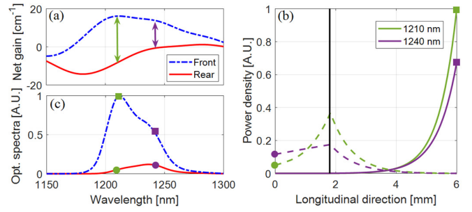
Fig.3. Simulations. (a) Net optical gain close to the front facet (dot-dashed blue line) and the rear facet (continuous line). Arrows indicate the net gain difference at 1210 nm and 1240 nm. (b) Longitudinal distribution of the photons at 1210 nm and 1240 nm propagating in the forward (continuous lines) and backward (dashed lines) directions. The vertical black line indicates the separation between the two electrodes. (c) Resulting optical spectra. Markers in (b) and (c) indicate the same points.
