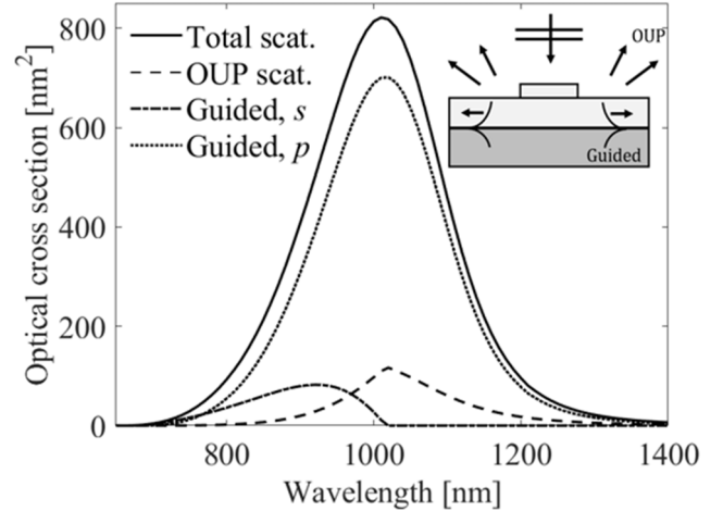
Fig. 2. Scattering cross section spectrum for light normally incident on a geometry with a cylindrical scatterer (radius 30 nm and height 25 nm) on top of a 50-nm-silicon-film-on-silver waveguide. The scattering cross section is divided into contributions s - and p -polarized guided modes, and out-of-plane scattering.
