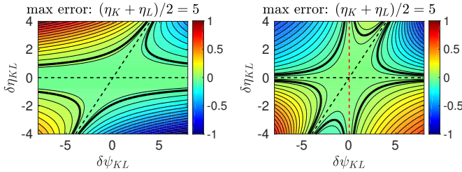
Fig. 1. Logarithmic absolute errors between the generalized Scharfetter-Gummel and the diffusion enhanced scheme (left) and the Sedan scheme (right) for \bar{\eta}_{KL} = 5 .
