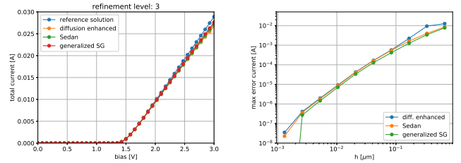
Fig. 2. Left: The I-V curves computed with the different schemes for fixed mesh refinement. The reference solution was computed using the generalized Scharfetter-Gummel scheme on refinement level 10. Right: Convergence studies for the absolute errors of the total currents.
