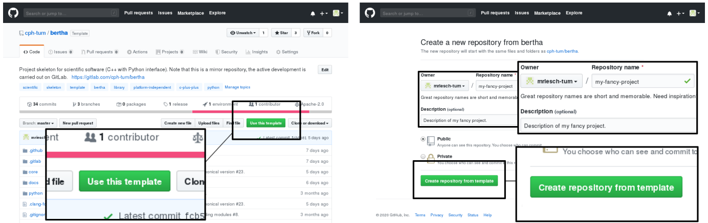
Fig. 1. Creating an instance of bertha on GitHub. On bertha's project page [11], click on "Use this template" and enter the desired owner, repository name, and project description. The button "Create repository from template" will then create the instance. Reprinted from M. Riesch et al. [10] (CC BY 4.0).
