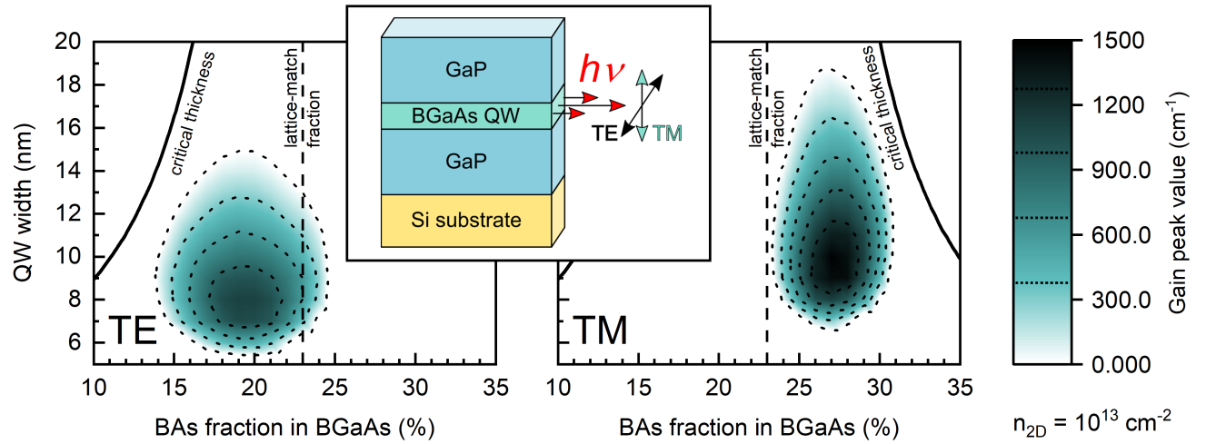
Fig. 1. Peak gain of quantum wells at room temperature in function of the QWs width and BAs mole fraction, schematics of the epitaxial structure consisting a single GaP/B x Ga 1-x As/GaP quantum well.
