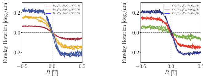
Fig. 2. FR hysteresis loops of Bi:YIG/YIG and YIG/Bi:YIG bilayers deposited on Si substrates.
