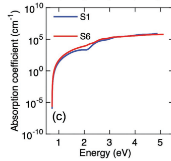
Fig. 3. Spectral dependence of absorption coefficient of YIG/Bi 0.8 YIG (blue) and Bi 1.5 /YIG (red) bilayers on Si substrate [9].
