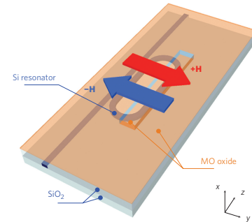
Fig. 1. Scheme of the nonreciprocal optical resonator structure [6].
