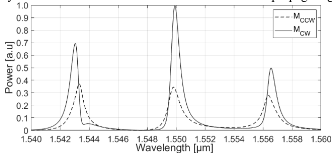
Fig. 3. Emission spectra relative to the simulation of the launch configuration shown in Fig. 2a. The CCW and CW field are measured from the monitors M_{CCW} and M_{CW} , respectively.
