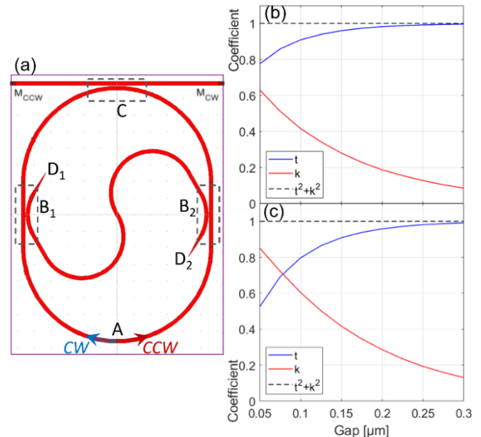
Fig. 1. (a) RSoft schematic of the consider racetrack and a S-shaped waveguide. (b,c) Coupling and transmission coefficients at \lambda=1.55 \mu\text{m} as a function of the coupler gap for the directional couplers B_1 and B_2 (b) and the directional coupler C (c).
