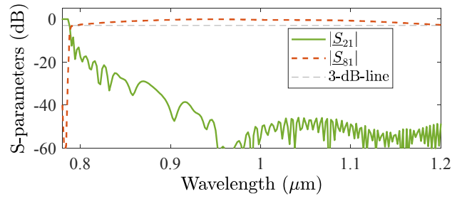
Fig. 3. The S-parameters of the presented system from Fig. 1(b) are illustrated. An ER of 60 dB can be realized. Signals with wavelengths between 790 nm and 1200 nm transmit with lower attenuation than 3 dB to port 8. This results in a 3-dB bandwidth of more than 400 nm. The reflected signal can be coupled out from port 2.
