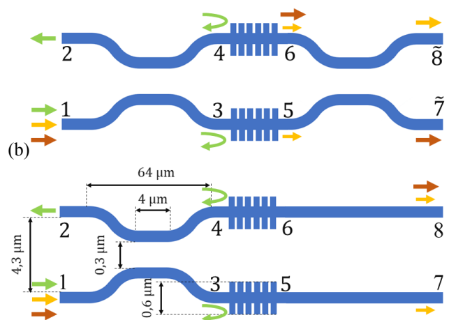
Fig. 1. In (a) a common setup of the filter system is shown. A 3-dB coupler realized by a DC splits the incident signal equally among the outgoing arms. Each BG in the corresponding arm reflects the green marked signals, which fulfill the Bragg conditions. The reflections pass the first 3-dB coupler again and interfere constructively at port 2 and destructively at port 1. Signal parts with longer wavelengths (orange and red) pass the BGs nearly undamped and are combined again by another 3-dB coupler. In (b) a proposed setup with improved frequency characteristic in the passband is presented.
