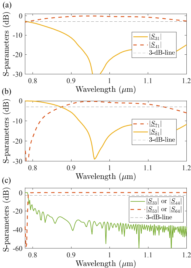
Fig. 2. Simulation results for single components of the filter. In (a) the scattering parameters (S-parameters) of the designed DC are shown. For the considered range of wavelength, the power couples mainly to the crossed waveguide. The transmissions to the output ports 7 and 8 of a MZI, build up as depicted in Fig. 1(a) omitting the BGs, results to (b). Due to the deviation of the 3-dB characteristic of the DCs for longer wavelengths, the signals leaving port 8 show a transmission over 3 dB up to 870 nm only. The reflection and transmission of a designed BG are shown in (c). At the CW at 785 nm an ER of 60 dB and a FWHM around 10 nm are achieved.
