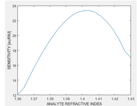
Fig. 6. The Sensitivity versus the change of refractive index
