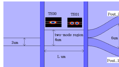
Fig. 2. The layout dimensions of biosensor for BPM computational simulation and two-dimensional mode profiles in the two-mode region for the cladding refractive index, 1.33.
