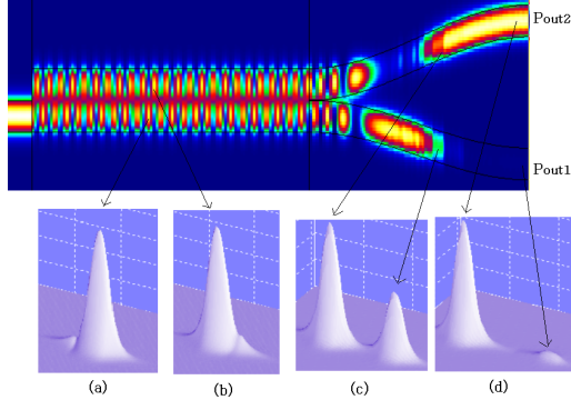
Fig. 3. Power coupling between two modes along propagation and mode evaluations in two-mode region and output waveguides
