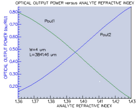
Fig. 4. The normalized two output power intensity versus the change of refractive index.
