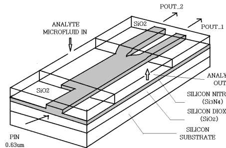
Fig. 1. The layout of biosensor based on \text{Si}_3\text{N}_4 rib-optical waveguides.
