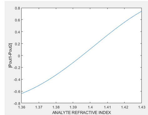
Fig. 5. The difference |P_{out1} - P_{out2}| of normalized two output power intensity versus the change of refractive index.
