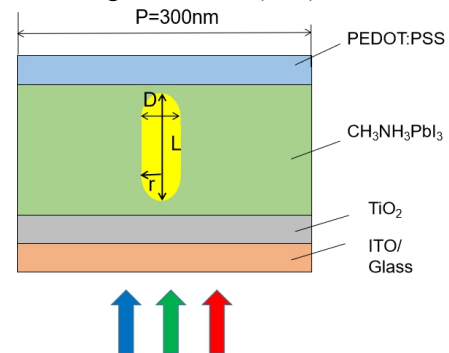
Fig. 1. Schematic of plasmonic perovskite solar cells embedding Ag nanorods
