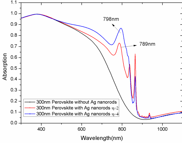
Fig. 2. Absorption spectrum of plasmonic perovskite layer ebedding Ag nanorods versus length-diameter ratio
