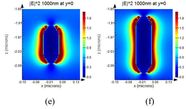
Fig. 3. Electric intensity distribution at the cross section of plasmonic perovskite layer ebedding Ag nanorods versus length-diameter ratio (a) \eta=2 , \lambda=650\text{nm} ; (b) \eta=4 , \lambda=650\text{nm} ; (c) \eta=2 , \lambda=789\text{nm} ; (d) \eta=4 , \lambda=798\text{nm} ; (e) \eta=2 , \lambda=1000\text{nm} ; (f) \eta=4 , \lambda=1000\text{nm} .
