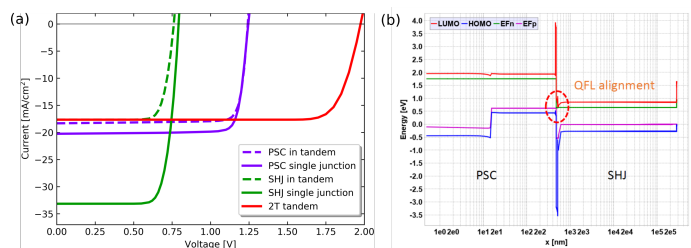
Fig. 4. (a) Current-voltage characteristics from full opto-electronic simulations of perovskite (PSC) top- and silicon heterojunction (SHJ) bottom cells in single junction configuration, as well as of the corresponding tandem device. (b) Band profile (log scale position axis) at MPP exhibiting the absence of a voltage drop at the recombination junction, which is reflected in the perfect alignment of electron and hole quasi-Fermi levels (QFL).
