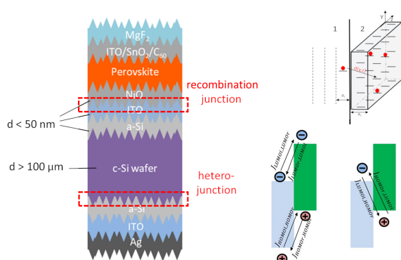
Fig. 2. Regarding the challenges for electrical simulation, the perovskite-silicon tandem device exhibits large disparity in the thickness of the component layers, and several hetero-interfaces, with either intra- or interband charge transfer. The latter is simulated here by an interface hopping model similar to the Miller-Abrahams theory for thermally activated transport.
