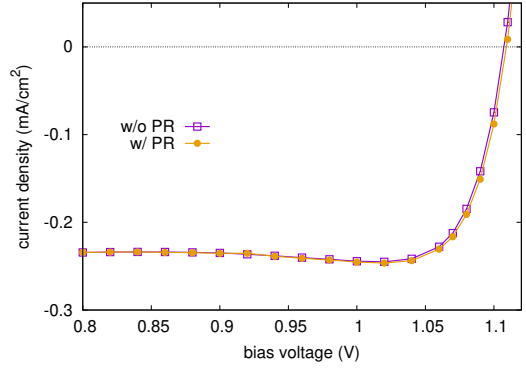
Fig. 3. Current-voltage characteristics of a 50 nm GaAs p-i-n solar cell, with PR (full symbols) and without PR (empty symbols). The additional generation from reabsorption results in a V_{OC} enhancement of about 2 mV. The peculiar shape of the curve around MPP is due to the bias dependence of the photocurrent.
