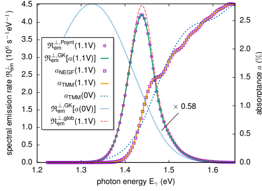
Fig. 2. Absorbance and front-side emission of a 100 nm GaAs p-i-n solar cell with gold rear reflector, reflecting the impacts of built-in field variation and reabsorption [7].
