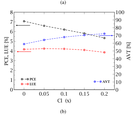
Fig. 2. (a) JV curves (full-lines) obtained with DD simulations by varying x ; the dotted line represents the experimental curve considered as reference for the full study. (b) AVT, PCE and LUE obtained for Cl doping.
