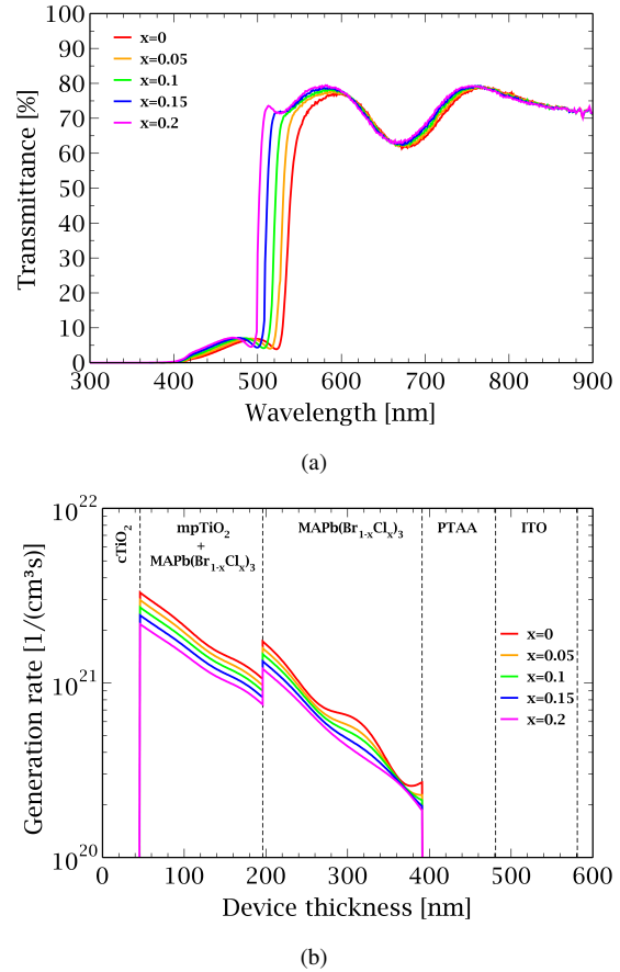
Fig. 1. Transmittance (a) and internal generation profile (b) obtained with TMM calculations by varying the chlorine doping from 0 to 0.2.
