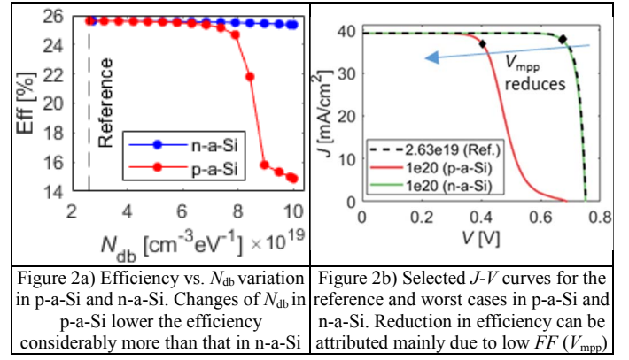
Figure 2a) Efficiency vs. N_{db} variation in p-a-Si and n-a-Si. Changes of N_{db} in p-a-Si lower the efficiency considerably more than that in n-a-Si. Figure 2b) Selected J - V curves for the reference and worst cases in p-a-Si and n-a-Si. Reduction in efficiency can be attributed mainly due to low FF ( V_{mpp} )
