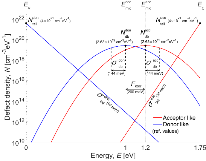
Figure 1 Defect state distribution in p-a-Si with stated reference values. The black symbols show the N_{db} parameters we have varied.
