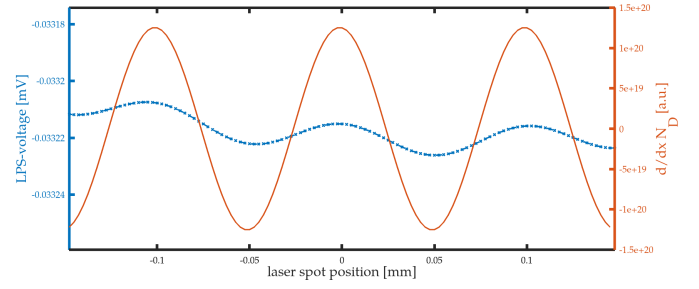
Fig. 3. Alignment between gradient of doping concentration and LPS voltage for a laser beam sampling along the x axis.
