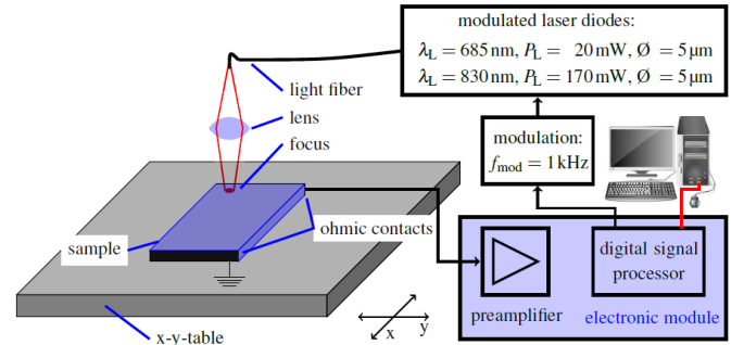
Fig. 2. LPS measurement setup.
