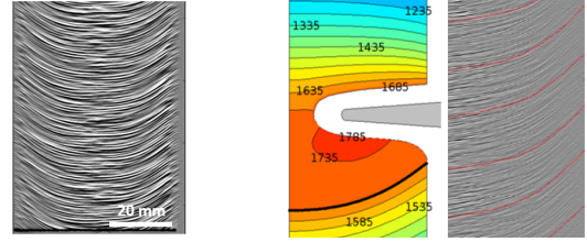
Fig. 1. Striations from LPS measurement (left); temperature field simulation of floating zone silicon crystal as well as striations (right). Here the black line represents the solid-liquid interface at 1687 K, leading to striations (tracked red line). Temperature field simulation by Robert Menzel (IKZ).
