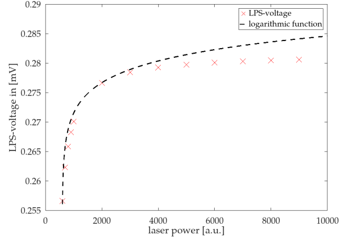
Fig. 4. Logarithmic behavior of LPS voltage as a function of the laser power. Our simulation matches the theoretic predictions made by Tauc [3].
