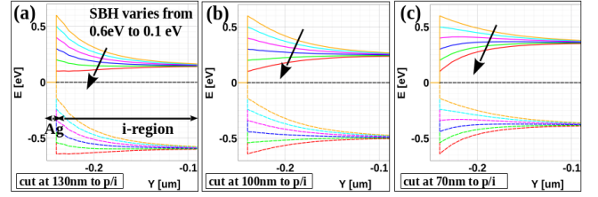
Fig. 5: (a)/(b)/(c) Band diagrams at Schottky interface in plasmonic device with varying SBHs in dark at 0 V, obtained by a vertical cut at 130nm/100nm/70nm far from p/i junction. Colored solid (dashed) and black dashed lines represent CB (VB) edge and Fermi level.
