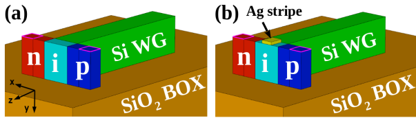
Fig. 1: Sketch of the (a)/(b) non-plasmonic/plasmonic device.
