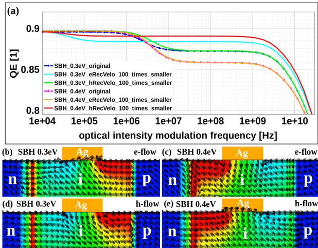
Fig. 4: (a) Frequency response curves of the plasmonic device with a SBH of 0.3 eV and 0.4 eV, together with curves obtained from reference studies using scaled (100 times smaller) thermionic emission velocities of carriers. (b)/(c) Electron and (d)/(e) hole current vector plot in the plasmonic device with a SBH of 0.3/0.4 eV under light at -2 V, obtained by a vertical cut along p-i-n at 100 nm distance to i/Si. Background contour profile represents the corresponding E-field, with color bar from blue to red ranging from 0 to 3 \times 10^5 V/cm.
