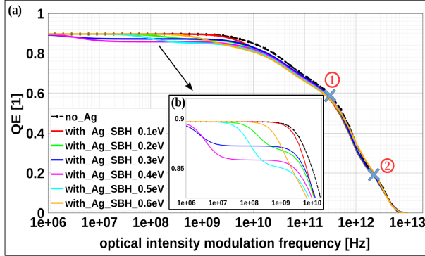
Fig. 3: (a) Comparison of frequency response curves of non-plasmonic and plasmonic devices with SBHs ranging from 0.1 eV to 0.6 eV. A zoomed-in plot is depicted in insertion (b).
