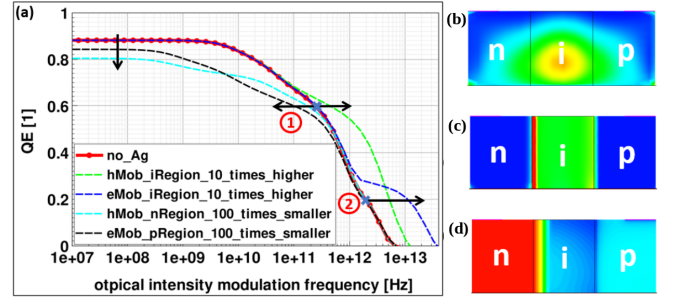
Fig. 2: (a) Frequency response curve of a non-plasmonic device and curves obtained with scaled carrier mobility from reference study. Optical generation rate (b), electric field (c) and electron density (d) profile at -2 V, obtained by a vertical cut in p-i-n direction at distance of 100 nm to the i/Si interface. Color bar from blue to red ranges from 0 to 2 \times 10^{23} \text{ cm}^{-3} \text{ s}^{-1} in (b), from 0 to 3 \times 10^5 \text{ V/cm} in (c) and from 3 \times 10^8 to 3 \times 10^{19} \text{ cm}^{-3} in (d).
