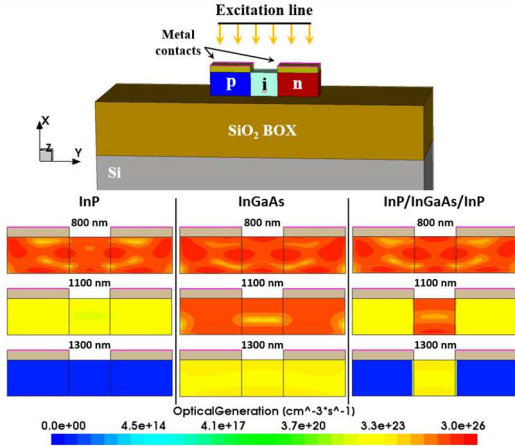
Figure 1: Top: sketch of the simulation domain together with the device geometry and source of light. Bottom: optical generation-coloured plots for each device.
