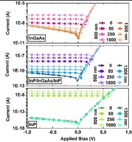
Figure 4: I-V curves for the three structures at four different laser powers (units of μW/μm 2 ) and two different wavelengths.
