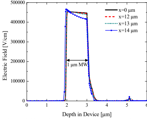
Fig. 2. Electric field as a function of depth at the center and near the edge ( x=12, 13 & 14\text{ }\mu\text{m} ) of the diffusion aperture corresponding to V = -50 V.
