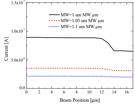
Fig. 4. Simulated photocurrent as a function of beam position corresponding to V = -50 V and for all three MW devices.
