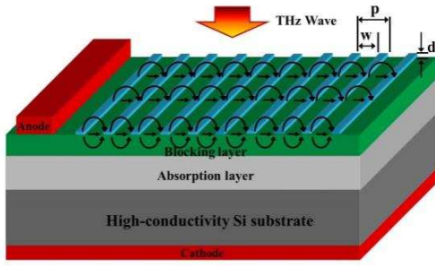
Fig.1. The schematic diagram of metal gratings/Silicon-based BIB THz detector.
