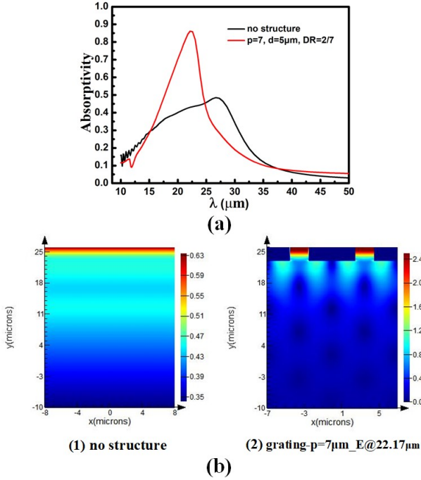
Fig.2. The absorption properties of the Si-based BIB device with metal gratings (parameters: p=7\mu\text{m} , d=5\mu\text{m} , DR=2/7 ) compared with that of device without metal gratings. (a) The absorption spectrum; (b) The longitudinal profile of of electric field intensity.
