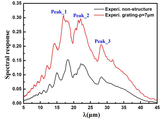
Fig.3. The experimental spectral response of device with metal gratings (parameters: p=7\mu\text{m} , d=5\mu\text{m} , DR=2/7 ) compared with that of device without metal gratings.
