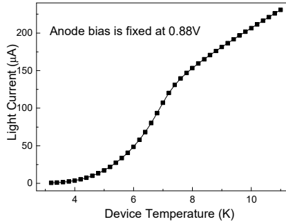
Fig. 2. Temperature-dependent light current characteristics with device temperature decreasing from 11K to 3K in 0.2K steps.
