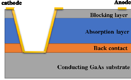
Fig. 1. The structure of GaAs-based BIB terahertz detector.
