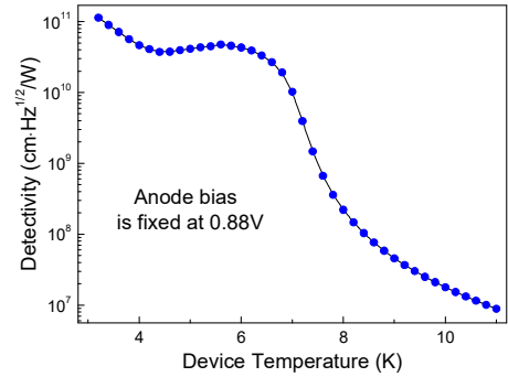
Fig. 4. Characteristic curve of the detectivity of GaAs BIB terahertz detector as a function of device temperature
