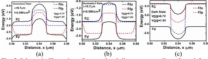
Fig. 3 Schematic illustration of energy band diagram uncoupling of quasi Fermi levels at the illumination state ( I=0.5\text{W/cm}^2 and \lambda=0.7\mu\text{m} ) along the line AA' (a) near gate-oxide interface (b) top surface of optical gate (c) under take state.
