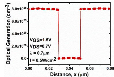
Fig. 2 Optical generation at gate region.
