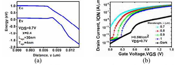
Fig. 4 (a) Energy band diagram at ON state. (b) Transfer characteristics plots at different wavelength
