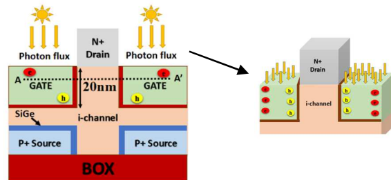
Fig. 1 Schematic illustration of optically gated Dual MOSCAP VTFET for photosensing application.
