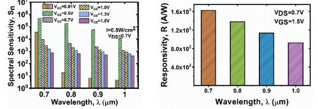
Fig. 5 (a) Spectral sensitivity for different wavelength. (b) corresponding Responsivity at V_{GS}=1.5\text{V} .
