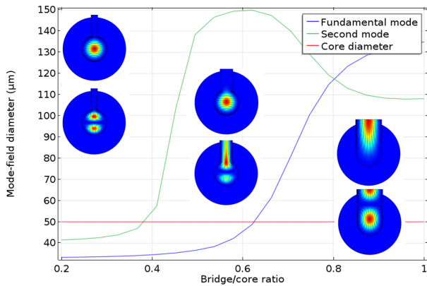
Fig. 2. 2D cross-section simulation of the first two supported modes of a bridged optical through-silicon waveguide. The mode-field diameter of the fundamental and the second supported modes are plotted versus the bridge-to-core size ratio. In addition, the normalized electrical field for the first two modes in the three different regions is shown.
