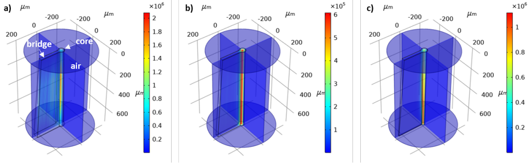
Fig. 1. 3D beam propagation simulation of a bridged optical through-silicon waveguide with a tapering angle of a) -0.9^\circ , b) 0^\circ and c) 0.9^\circ . The surrounding substrate is hidden and the electric field values are represented on the x, y and z planes.
