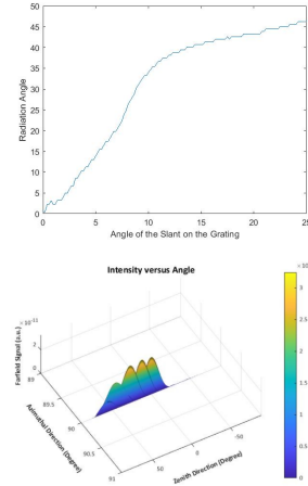
Figure 4. a) Slanted angle vs Radiation Angle; b) Farfield pattern from Slanted Grating Coupler.
