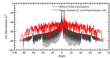
Figure 2. Simulated OPA far field pattern for edge-fire emitters; black) far field Intensity without random phase and phase gradient; red) far field with steering for random phase and a phase gradient of 20^\circ .
