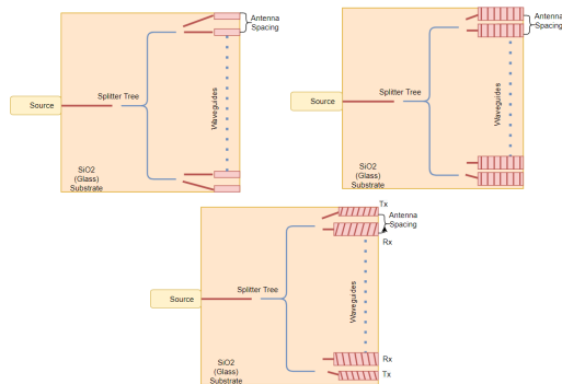
Figure 1. a) Edge-fire system; b) Grating Coupler System; c) Slanted Grating Coupler System
