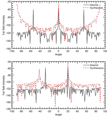
Figure 3. a) Farfield desired vs synthesised; b) Steering range.
