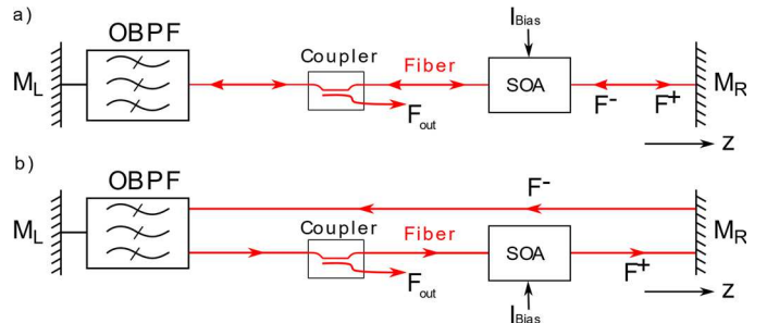
Fig. 1. a. Bidirectional SOA Fiber Laser Cavity b. One-way SOA Fiber Laser Cavity L_1=9\text{m} and L_2=1\text{m} in our simulation
