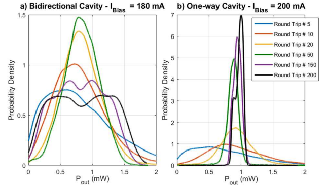
Fig. 3. Probability density function of P_{out}(t)
