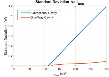
Fig. 4. Standard Deviation vs I_{Bias} for Bidirectional and One-way Cavities.
