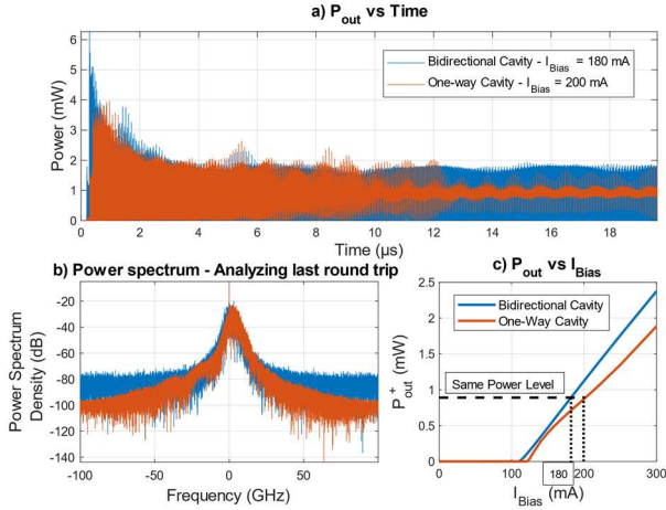
Fig. 2. a. Time domain analysis of 165 round trips for different I_{bias} and cavity structures. b. Frequency analysis for the last round trip (steady state). c. P_{out} vs I_{Bias} for Bidirectional and One-way Cavity.
