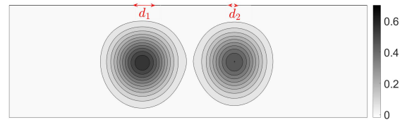
Fig. 2. Cross section of two waveguides manufactured with a field-assisted ion exchange from different mask opening widths d_1 and d_2 .
