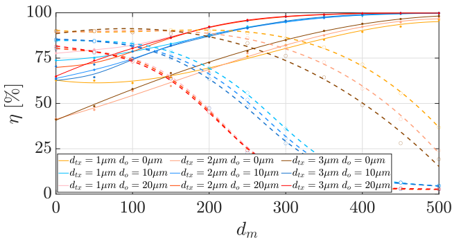
Fig. 3. Calculated efficiencies in receiving direction (RX, continuous) and transmitting direction (TX, dashed) that is depending on various optimization parameters.
