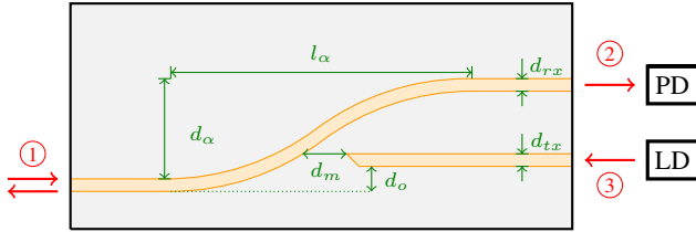
Fig. 1. Mask design of an S-bend with a branching and the optimization approaches of mask bridge d_m , coupling angle \alpha and mask opening width of the transmitting branch d_{tx} .
