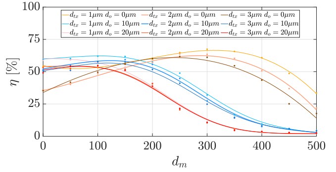
Fig. 4. Calculated overall efficiency \eta that is derived by a multiplication of the efficiencies \eta_{rx} and \eta_{tx} in both directions.
