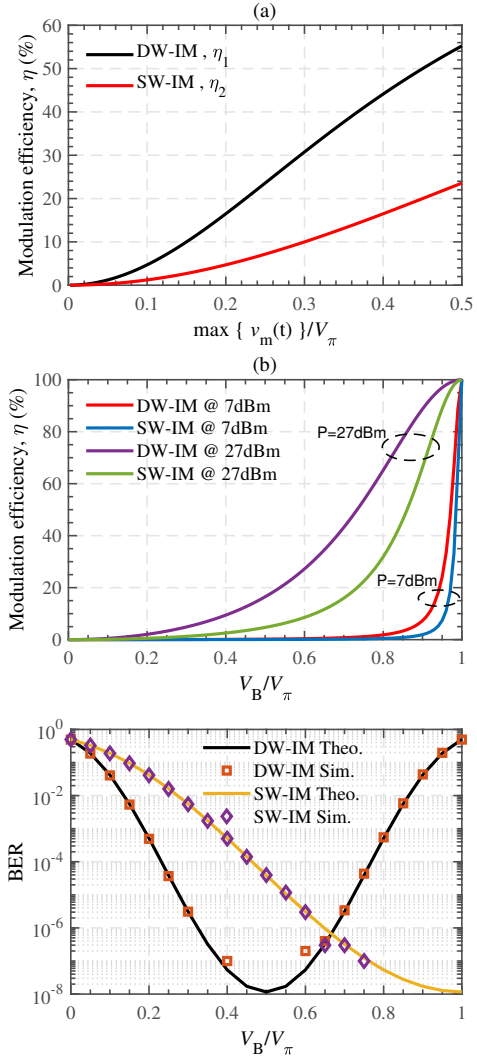
Fig. 2. Modulation efficiency for a single tone driving signal in both configurations versus (a) the modulating signal amplitude and (b) the MZM bias voltage. (c) Bit error rate performance of OOK modulation with both configurations. DW: dual wavelength. SW: single wavelength. Theo.: theoretical. Sim.: simulations.
