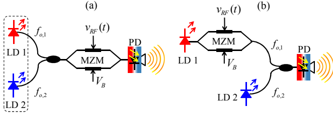
Fig. 1. Two possible topologies for millimeter wave photonic generation techniques. (a) the DW-IM topology. (b) SW-IM topology.
