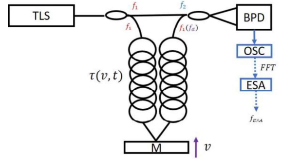
Fig. 1: System diagram of onchip FMCW doppler LiDAR system.
