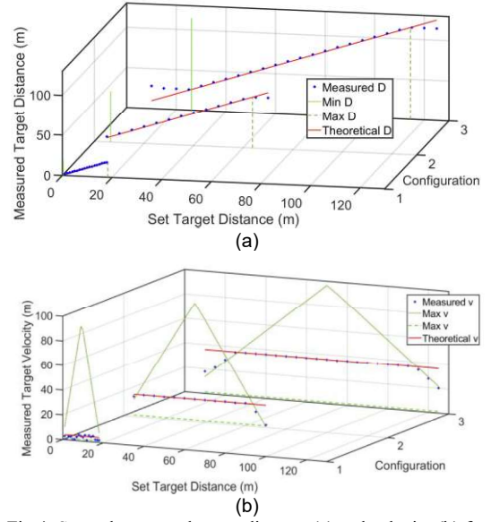
Fig.4: Set and measured target distance (a) and velocity (b) for three different configurations.
