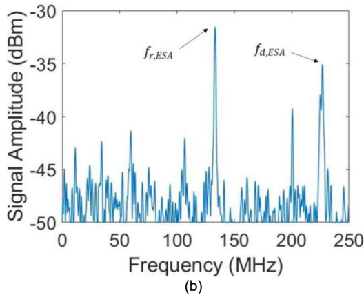
Fig. 3: Simulation result for configuration 1. Mixed signal detected on balanced detector (a) and spectrum (b).
