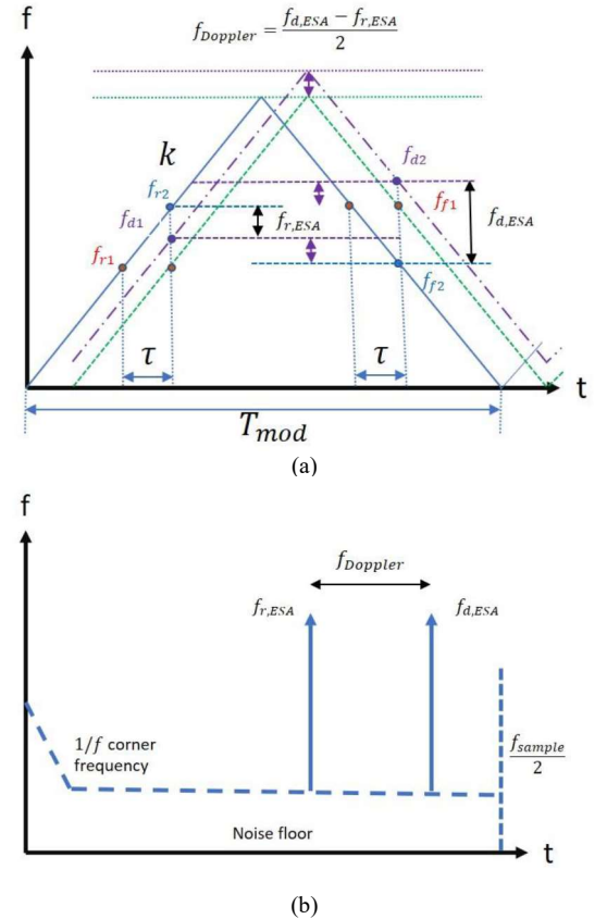
Fig. 2: Laser triangular wave modulation pattern and the delayed reflected signal (a). ESA spectrum (b).
