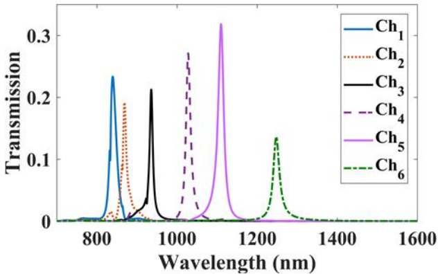
Fig. 4. Output spectrum of the proposed 6-channel DMUX.
