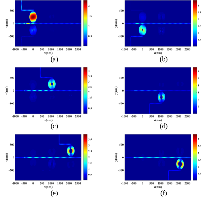
Fig. 5. Electric field intensity distributions of the proposed 6-channel DMUX for resonance wavelengths of (a) \lambda_1=840\text{nm} , (b) \lambda_2=869\text{nm} , (c) \lambda_3=936\text{nm} , (d) \lambda_4=1028\text{nm} , (e) \lambda_5=1110\text{nm} , and (f) \lambda_6=1248\text{nm} .
