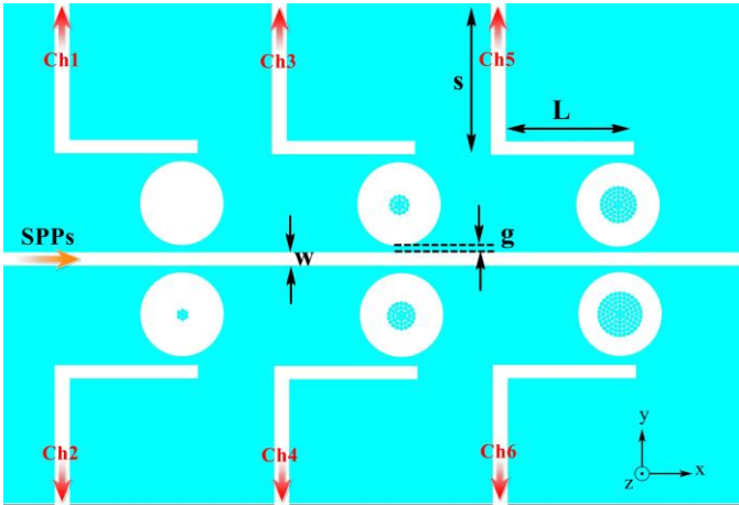
Fig. 3. The designed 6-channel DMUX with six CRs consisting of different rows of NRAs.
