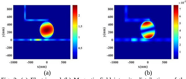
Fig. 2. (a) Electric and (b) Magnetic field intensity distributions of the 1-channel structure at resonance wavelength of \lambda=840\text{nm} .
