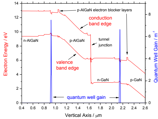
Fig. 2: Electron energy band edges (red) and quantum well gain (blue) calculated at 2A input current.
