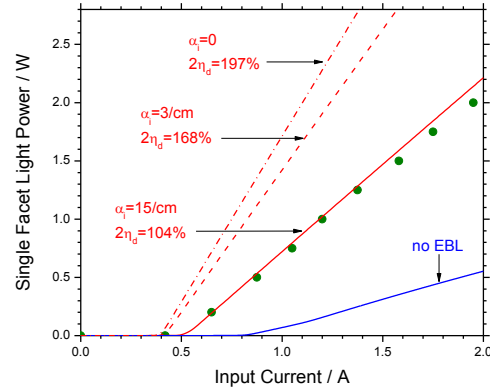
Fig. 3: Simulated output power vs. current with varied modal absorption \alpha_i (red lines, \eta_d – differential quantum efficiency). Symbols show measured data. 6 The blue line is calculated without electron blocker layer (EBL).
