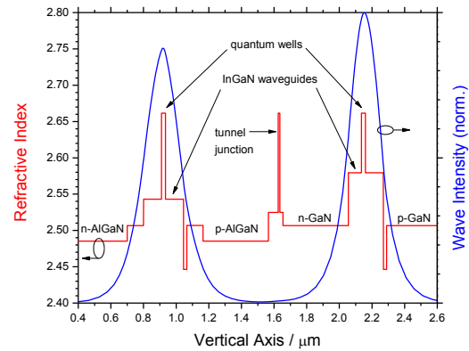
Fig. 1: Vertical profiles of refractive index (red) and lasing modes (blue).
