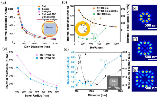
Fig. 2(a) Thermal resistance of disk, square and hexagon microcavity dependent on diameter; (b) and (c) thermal resistance of ring cavities dependent on ring parameter; (d) Experimental threshold versus diameter of InP whispering gallery mode cavities and simulated mode volume fractions. (e)-(g) Simulated resonant modes corresponding to the mode volumes in (d) with diameters of 500 nm, 700 nm, 900 nm.
