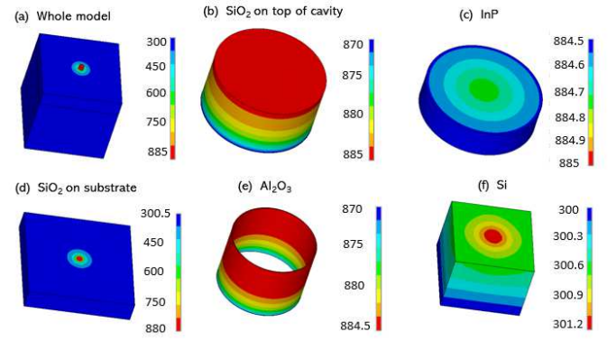
Fig. 3. Temperature profile of the micro-disk laser with diameter of 600 nm.
