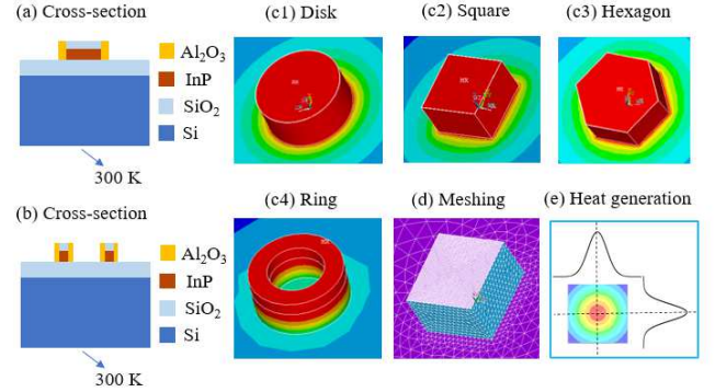
Fig. 1. The Schematic configuration (a) cross-section of (c1) disk (c2) square (c3) hexagon; (b) cross-section of (c4) ring; (d) meshing of square model; (e) gaussian distributed heat generation on square model. The thermal conductivity used in the simulation for Si, SiO 2 , InP and Al 2 O 3 is 131 W/m·K, 1.4 W/m·K, 68 W/m·K and 35 W/m·K, respectively.
