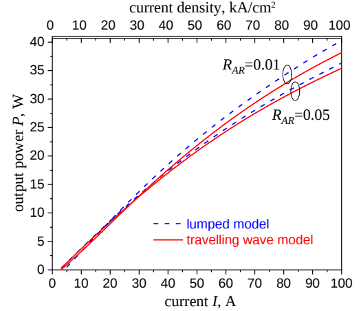
Figure 2. Output curves simulated with different models.
