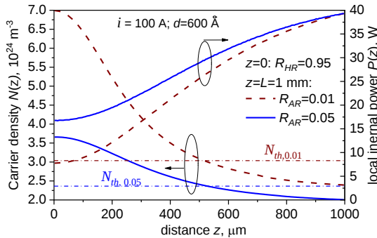
Fig. 1. Time-averaged P(z) and N(z) distributions along the 1 mm long cavity
