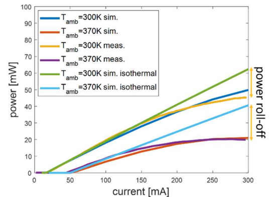
Fig. 3. OET TLLM simulated LI curves vs. measurements. The fitting of material parameters in the transmission line model is done in a similar way as in the physical simulation. The OET TLLM simulation provides good power roll-off accuracy using a fitted Lorentzian gain spectrum.
