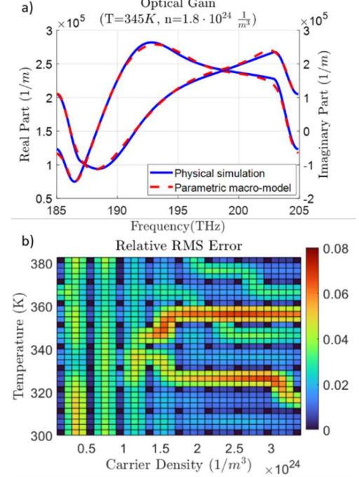
Fig. 5. Accuracy of the parametric macro-model for physical gain spectra: a) physical gain spectrum (solid) vs. parametric macro-model (dash) for a single (n, T) point. b) relative error of the parametric macro-model across the entire 2D parametric space (black squares indicate previously fitted training data).
