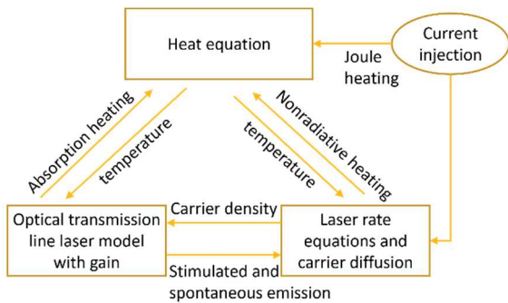
Fig. 1. Detailed coupling between the optical, electrical, and thermal subsystems, typical for physical simulations, can also be implemented in the time-domain transmission line laser model.
