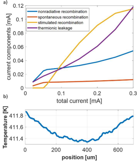
Fig. 4. OET TLLM also provides detailed outputs: a) contribution of different heat sources. b) position-dependent temperature profile along the laser cavity (small variation is due to the dominant contribution of Joule heating).
