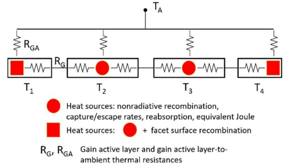
Fig. 2. Equivalent transmission line thermal model with a 4-section spatial laser discretization. The heat equation is self-consistently coupled to the OE equations to solve for section temperatures.
