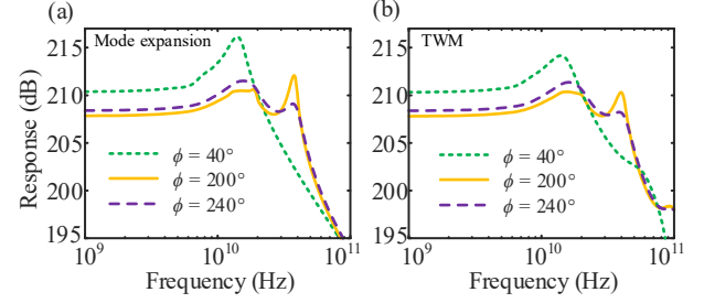
Fig. 4 Modulation responses calculated by (a) mode expansion method, and (b) TWM.
