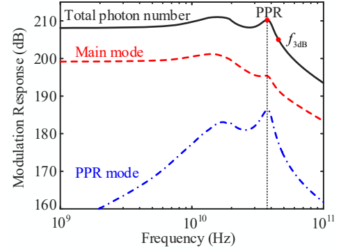
Fig. 3 Modulation responses of the photon number in the main mode, PPR mode, and the total photon number ( \phi = 220^\circ ).
