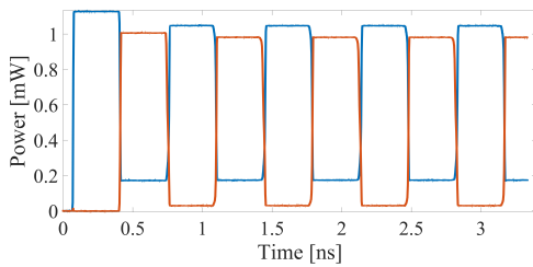
Fig.3 Mode switching in Regime I ( L_1 = 100 \mu\text{m} , L_2 = 5 cm)
