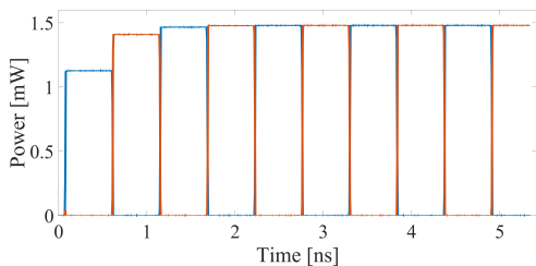
Fig.4 Mode switching in Regime IV ( L_1 = L_2 = 8 cm)
