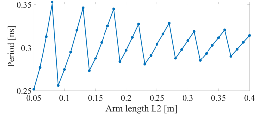
Fig.6 Linearity plot in Regime V ( L_1 = 2 cm)
