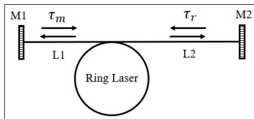
Fig.1 Ring laser subject to double delayed optical feedback
