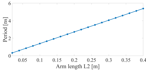
Fig.2 Linearity of Regime I ( L_1 = 100 \mu\text{m} )
