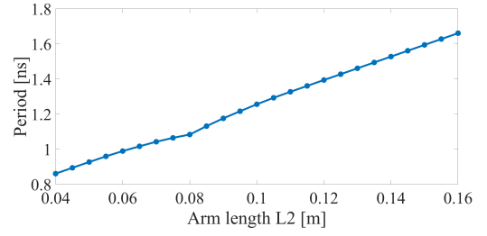
Fig.5 Linearity plot in Regime IV ( L_1 = 8 cm)
