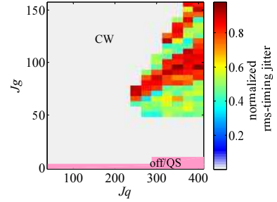
Fig. 5. The rms-timing jitter of PS that is normalized to the rms-timing jitter of WOICRS.
