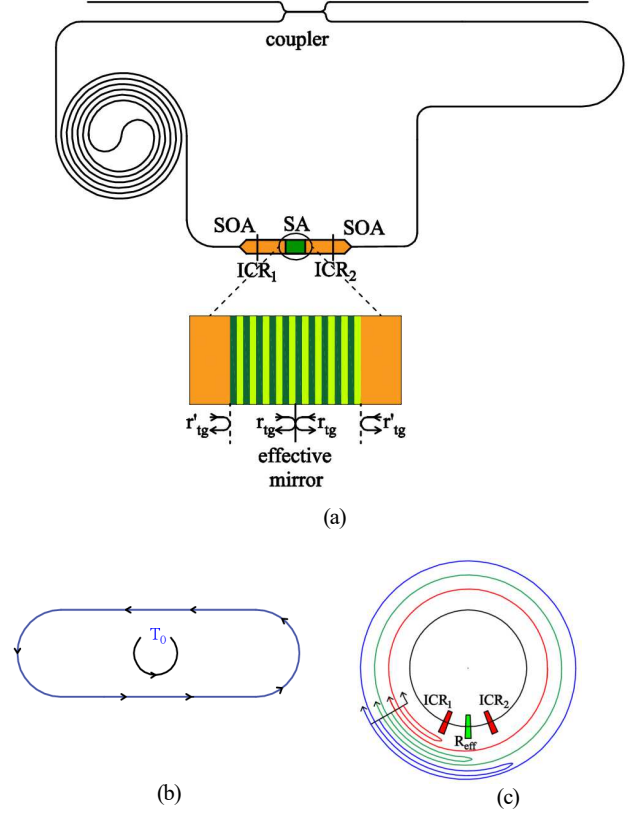
Fig. 1. (a) Schematic of proposed structure and corresponding paths for time delays used for derivation of DDE model in (b) WOICRS and (c) proposed structure.
