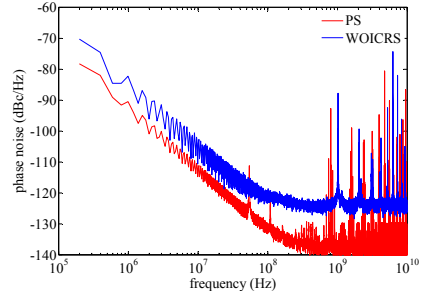
Fig. 4. The single side-band phase noise of PS and WOICRS.
