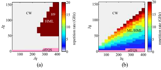
Fig. 2. Dynamic of repetition frequency for PS (a) WOICRS (b).
