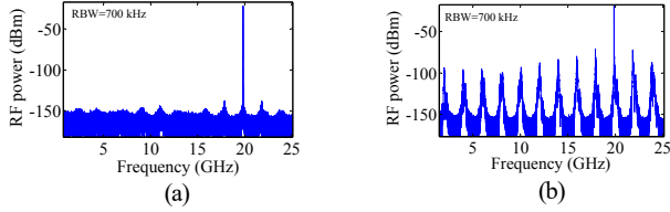
Fig. 3. Electrical spectrum (RBW=700 KHz) of 20 GHz harmonic regime of PS (a) and WOICRS (b).
