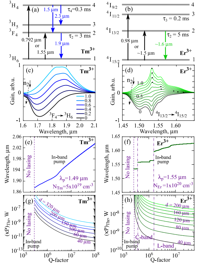
Fig. 1. Simplified schemes of energy levels of \text{Tm}^{3+} (a) and \text{Er}^{3+} (b). Normalized gain function proportional to (\sigma_{\text{em}}n_2 - \sigma_{\text{abs}}n_1) for \text{Tm}^{3+} (c) and \text{Er}^{3+} (d). Calculated laser wavelengths for in-band pumped microspheres doped with \text{Tm}^{3+} (e) and \text{Er}^{3+} (f). Threshold values of \kappa P_{\text{thr}} (pump powers multiplied by coupling coefficients) for different diameters of microspheres doped with \text{Tm}^{3+} (g) and \text{Er}^{3+} (h).
