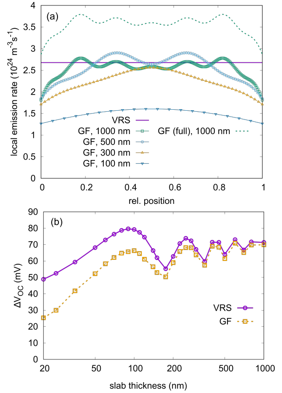
Fig. 1. (a) Local emission rate in a MAPI slab of different thicknesses, as compared to the spatially uniform VRS rate. (b) V_{OC} enhancement due to PR as a function of slab thickness, again compared to the result inferred from the VRS rate [10].
