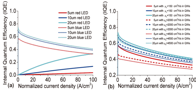
Fig. 2. (a) The IQEs of three kinds of chip size between red LED and blue \mu LED. (b) The influence of different carrier mobility in blue LED QWs with consideration on random alloy fluctuation.
