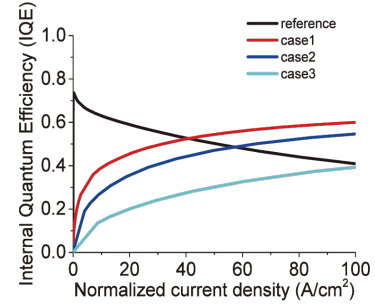
Fig. 3. Influence of different parameters to the IQE between blue LED and red LED. Reference is the case shown in Fig. 2(b) as cyan solid line. Case1 is the 20\mu\text{m} blue LED with \mu_n=4500\text{ cm}^2/\text{Vs} and \mu_p=190\text{ cm}^2/\text{Vs} in QWs. The random alloy potential fluctuation and piezoelectric polarization was removed. Case 2 is similar to case 1 but effective mass is set the same as red LED. Case 3 is further change the electron and hole mobility of QB to be \mu_n=4000\text{ cm}^2/\text{Vs} and \mu_p=180\text{ cm}^2/\text{Vs} , respectively.
