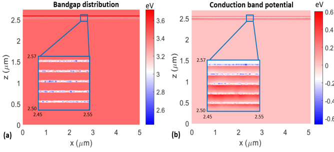
Fig. 1. (a) The bandgap distribution of the whole \mu LED with the random alloy fluctuation. The small picture is the enlargement of the InGaN LED quantum wells, where the composition fluctuation can be observed more clearly. (b) This is the conduction band potential of the whole \mu LED with the random alloy fluctuation. The small picture is the enlargement of quantum wells. The undulating potential is lead by inhomogeneous distribution of bandgap.
